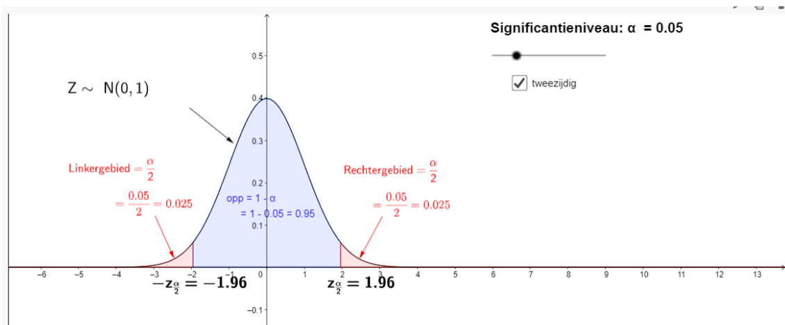
Figure 28: https://www.geogebra.org/m/gWCxY2Kt
