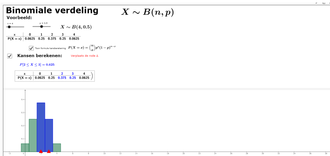
Figure 22: https://www.geogebra.org/m/Taz3435b
