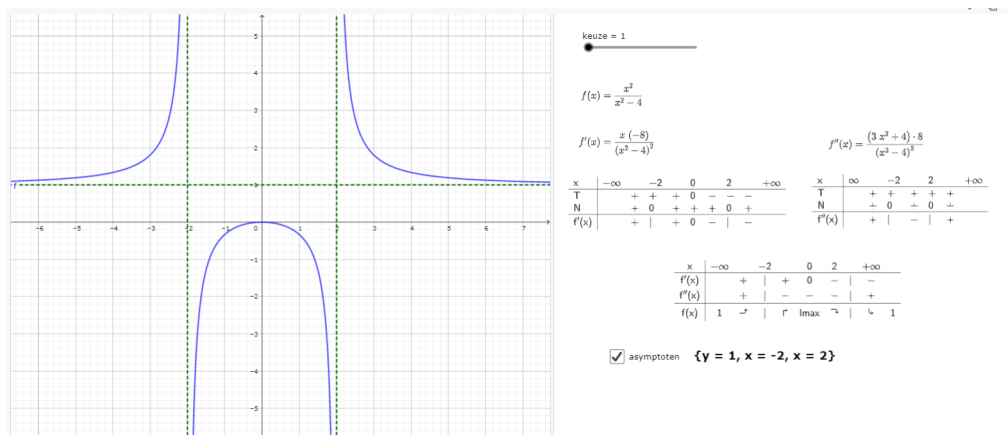
Figure 5: https://www.geogebra.org/m/gceq8KGM
