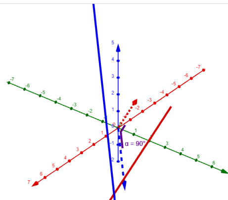
Figure 18: https://www.geogebra.org/m/furru9tk
