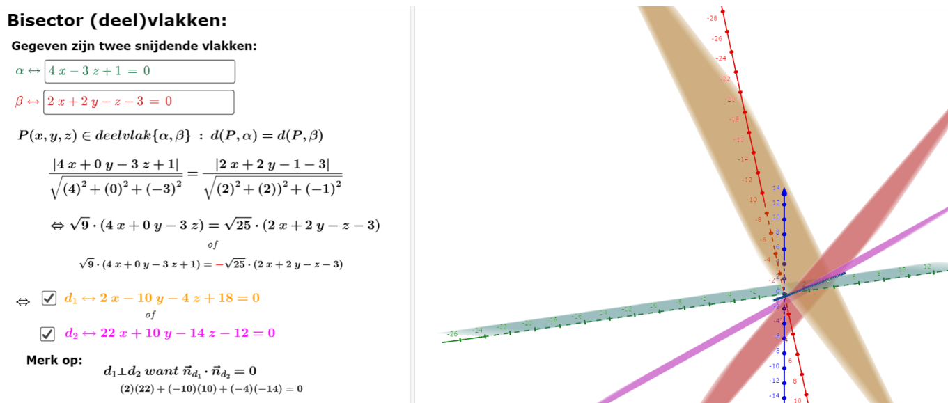
Figure 30: https://www.geogebra.org/m/jsffxvqd
