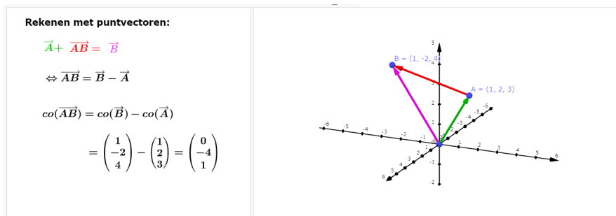
Figure 6: https://www.geogebra.org/m/msnt9fvp
